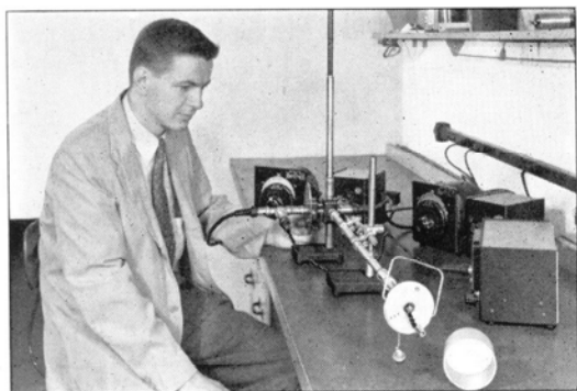
Admittance Meter set up with component mount and adjustable line to measure resistors at 500 megacycles.
