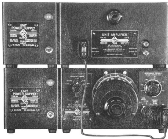
View of the TYPE 1206-A Unit Amplifier with the TYPE 1210-B Unit Oscillator. This combination delivers 3 watts over a range of 20 cycles to 50 kilocycles and 0.1 watt at 500 kilocycles.
