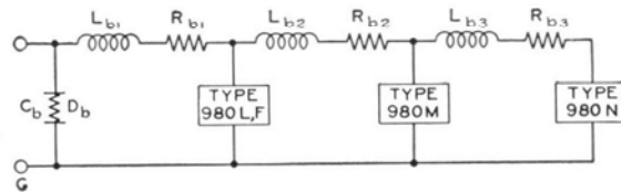
FIGURE 4. Equivalent circuit of a TYPE 219 Decade Condenser.
