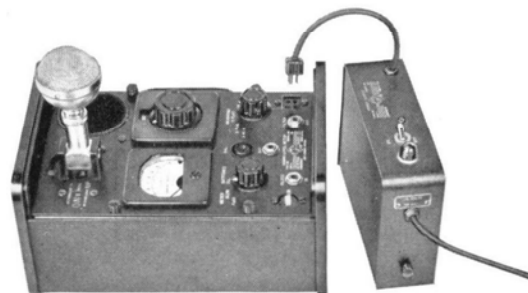
Batteries are furnished with the Sound-Level Meter. For a-c operation, the TYPE 1262-A Power Supply attaches to the sound-level meter cabinet, as shown above. For complete specifications, see page 147.
