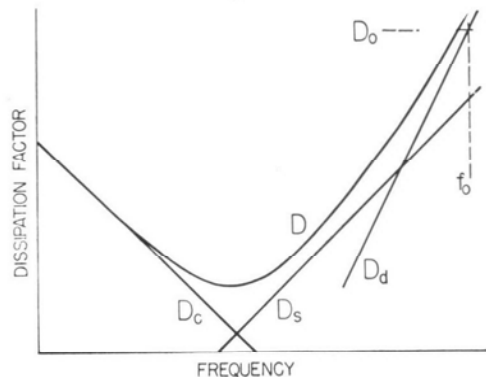
FIGURE B. Dissipation factor variation with frequency showing the relative contributions of the several components.
