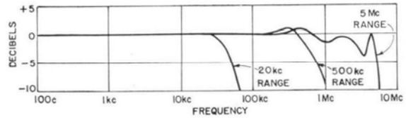
Typical Spectrum Level Characteristics for TYPE 1390-A Random-Noise Generator.
