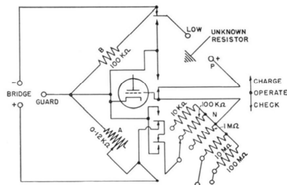
Schematic circuit diagram of the megohm bridge.
