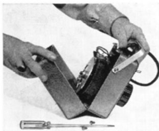
Cover of cased model is easily removable for access to terminals, mounting holes, and brush.
