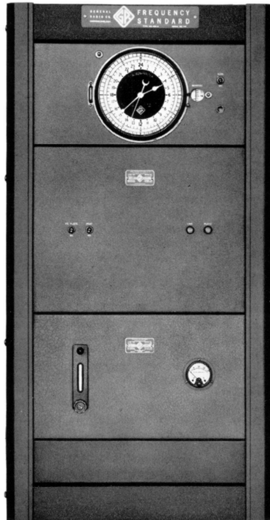
Close-up view of the TYPE 1100-AP Primary Frequency Standard. Lower part of the floor-type relay rack is not shown. The complete rack is similar to that shown in the photograph on page 77.
