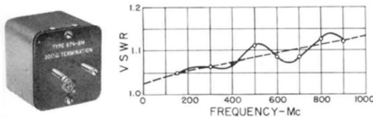
A plot of the VSWR as a function of frequency of a typical TYPE 874-BM 300-Ohm Balanced Termination Unit.
