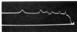
Oscillograms of the frequency characteristic of a TYPE 874-FR Rejection Filter tuned to 76 Mc. Sweep range is 48 to 250 Mc (upper) and 250 to 900 Mc (lower). Oscillator is driven by the TYPE 1750-A Sweep Drive; input amplitude is held constant by the TYPE 1263-A Amplitude-Regulating Power Supply. Vertical scale is square-law.
