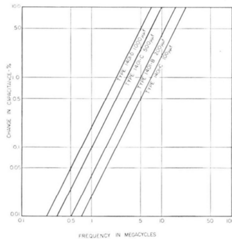
Variation with frequency of effective terminal capacitance due to residual inductance for each unit.
