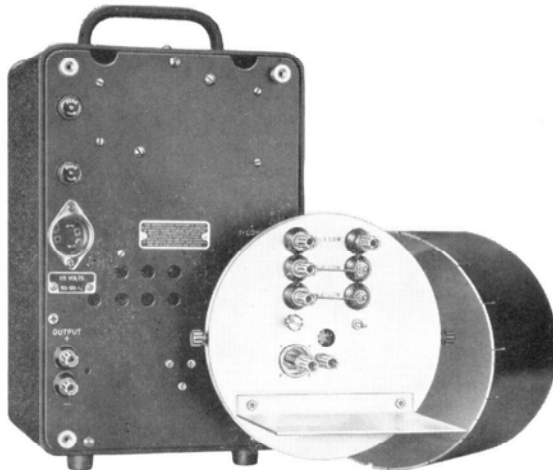
TYPE 1230-P1 Component Shield (with shield cover removed) plugged into the input terminal at the rear of the electrometer.
