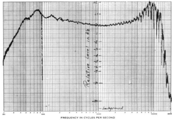
Graphic records of the frequency response of a tape recorder. Source was a TYPE 1304-B Beat-Frequency Audio Generator, driven by a TYPE 908-R96 X-Y Dial Drive. The vertical line at 100 cycles is the frequency calibration reference.
