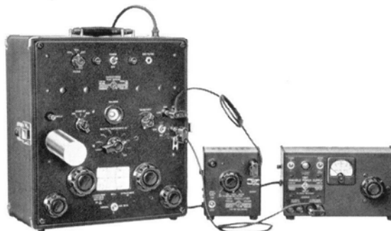
TYPE 1611-AS2 Capacitance Test Bridge used with the TYPE 1214-AS2 Oscillator to measure an electrolytic capacitor. The TYPE 1204-B Unit Variable Power Supply on the right supplies the d-c polarizing voltage.
