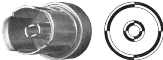
Figure 1. Photograph and, Figure 2, cross-section sketch of TYPE 874 Coaxial Connector.
