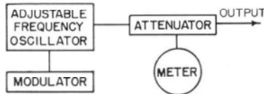
FIGURE 1. Elements of a standard-signal generator.
