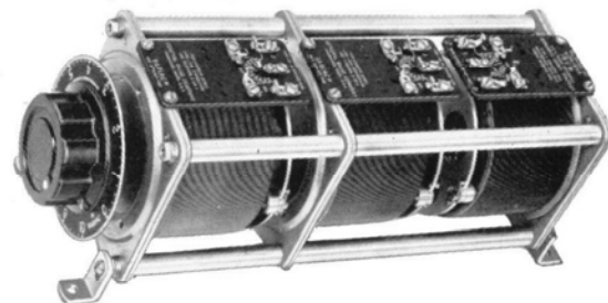
Right: A three-gang TYPE W5 Variac (TYPE W5G3). For photo of a cased W-model gang, see page 210. For a TYPE 50 gang, see page 214.
