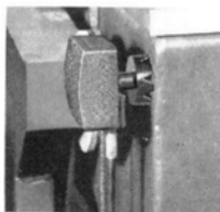
Vibration pickup held in place by the TYPE MAP-2-S1 Permanent-Magnet Clamp.
