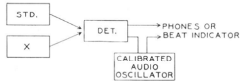
FIGURE 5. Functional diagram showing the operation of the direct-beating method of frequency measurement.
