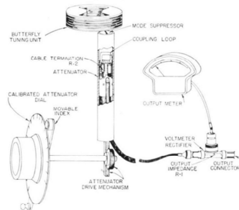
FIGURE 5. Functional diagram of the TYPE 1021-A output system.
