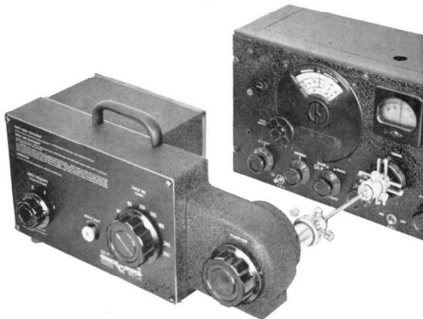
The sweep drive attached to the tuning knob of a short-wave receiver.
