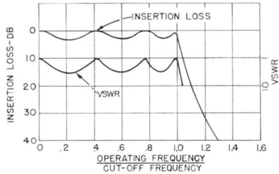
Insertion Loss and VSWR of the TYPE 874-F Low-pass Filters.
