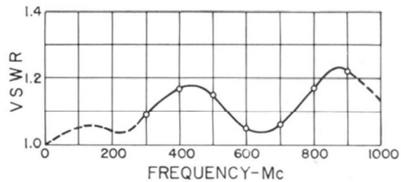
Plot of the VSWR at the 300-ohm terminals of a typical TYPE 874-UB-P3 Terminal Pad as a function of frequency when the pad is inserted in a properly adjusted balun whose coaxial circuit is terminated in 50 ohms.
