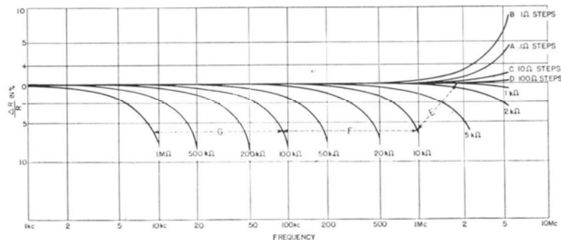
Maximum percentage change in series resistance as a function of frequency for TYPE 510 Decade-Resistance Units.
