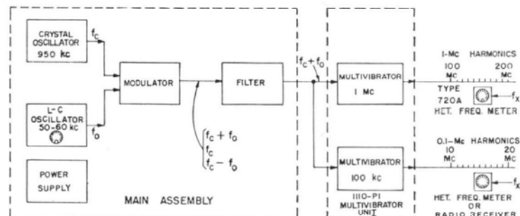
FIGURE 6. Block diagram showing the functional arrangement of the TYPE 1110-A Interpolating Frequency Standard.
