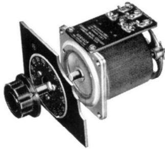
Type W2 Uncased Model. Mounting Base: 3¼ inches square. Depth Behind Panel: 3 15 / 16 inches. Four Mounting Holes on 2¾-inch square. Max. Panel: ⅜ inch.
